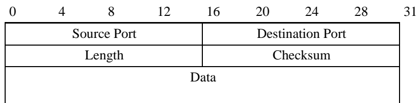
Figure 6-6 UDP Header Format
