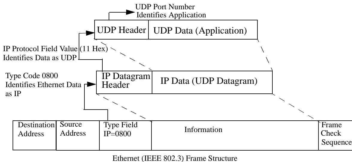
Figure 6-5 UDP Encapsulation
