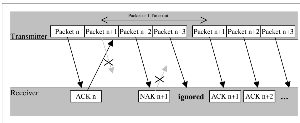
FIGURE 6.5 – “NAK PACKET LOST” TIME-OUT SCENARIO
