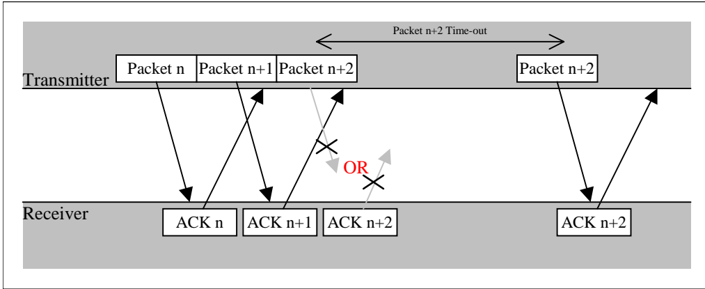
FIGURE 5.6 – “LAST PACKET LOST” TIME-OUT SCENARIO
