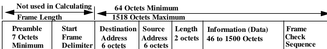
Figure 4.1 IEEE 802.3 Frame Structure
