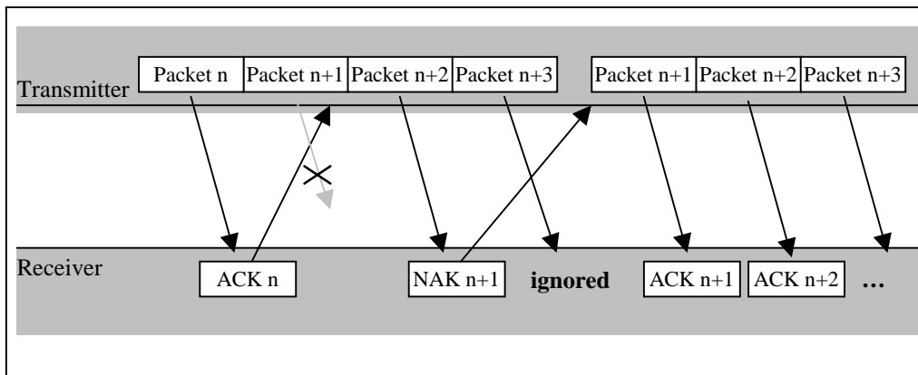
FIGURE 6.4 – OUT-OF-SEQUENCE RECEPTION
